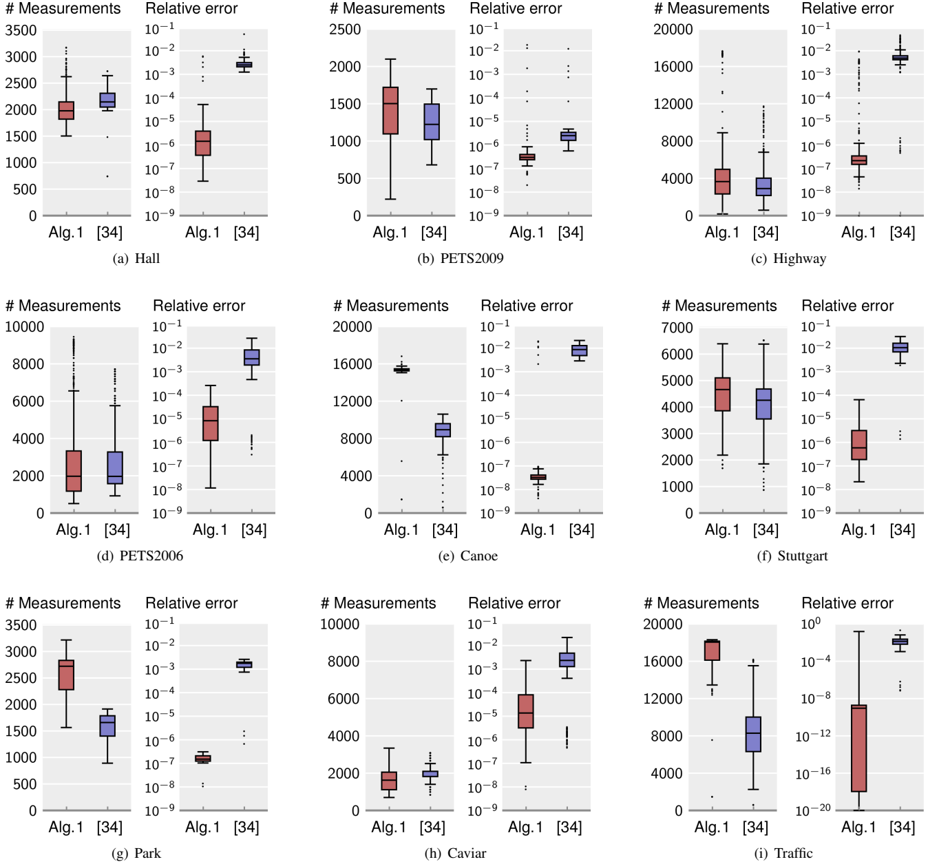
Figure 4. Results of Type II experiments. Each subfigure corresponds to a line of Table I and contains two boxplots: one for the number of measurements and another for the reconstruction error. In a boxplot, the horizontal line is the median, the box extremes are the Q_1 and Q_3 quartiles, and the whiskers are the minimum and maximum of data that is within 3/2 of the interquartile range of Q_1 and Q_3 ; points outside this range (outliers) are represented with dots.
