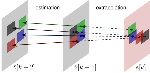
Figure 2. Scheme of motion-compensated extrapolation. We use the motion between matching blocks in \hat{z}[k-2] and \hat{z}[k-1] to create an estimate e[k] of frame z[k] .
