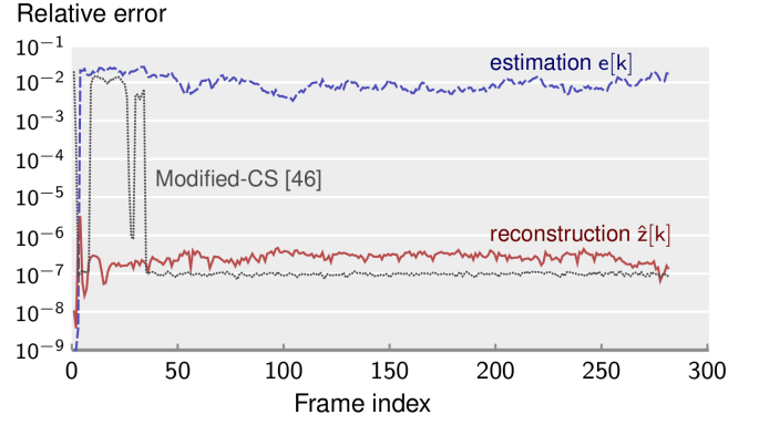
(b) Hall: Relative errors of estimation and reconstruction.
