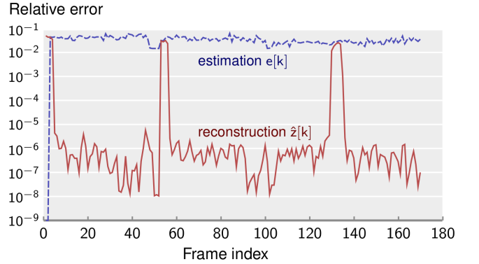
(f) PETS2009: Relative errors of estimation and reconstruction.
